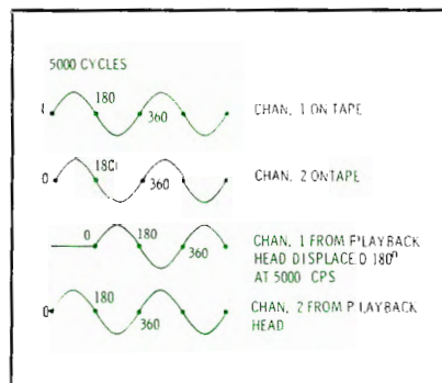
Fig. 2. Relation of 5-kc stereo signals.
