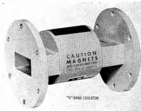
Fig. 3. One C-band ferrite isolator unit.
