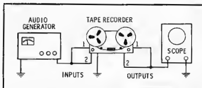
Fig. 4. Test setup for stereo alignment.
