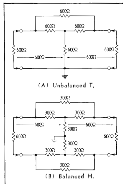
Fig. 6. Two six-decibel bridged networks.
