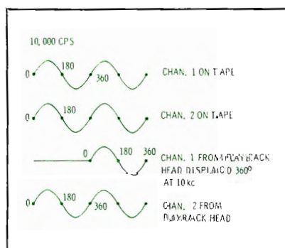
Fig. 3. Relation of 10-kc stereo signals.
