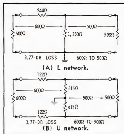
Fig. 9. Minimum loss, 600 to 500 ohms.
