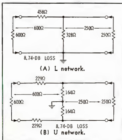
Fig. 8. Minimum-loss, 600 to 250 ohms.
